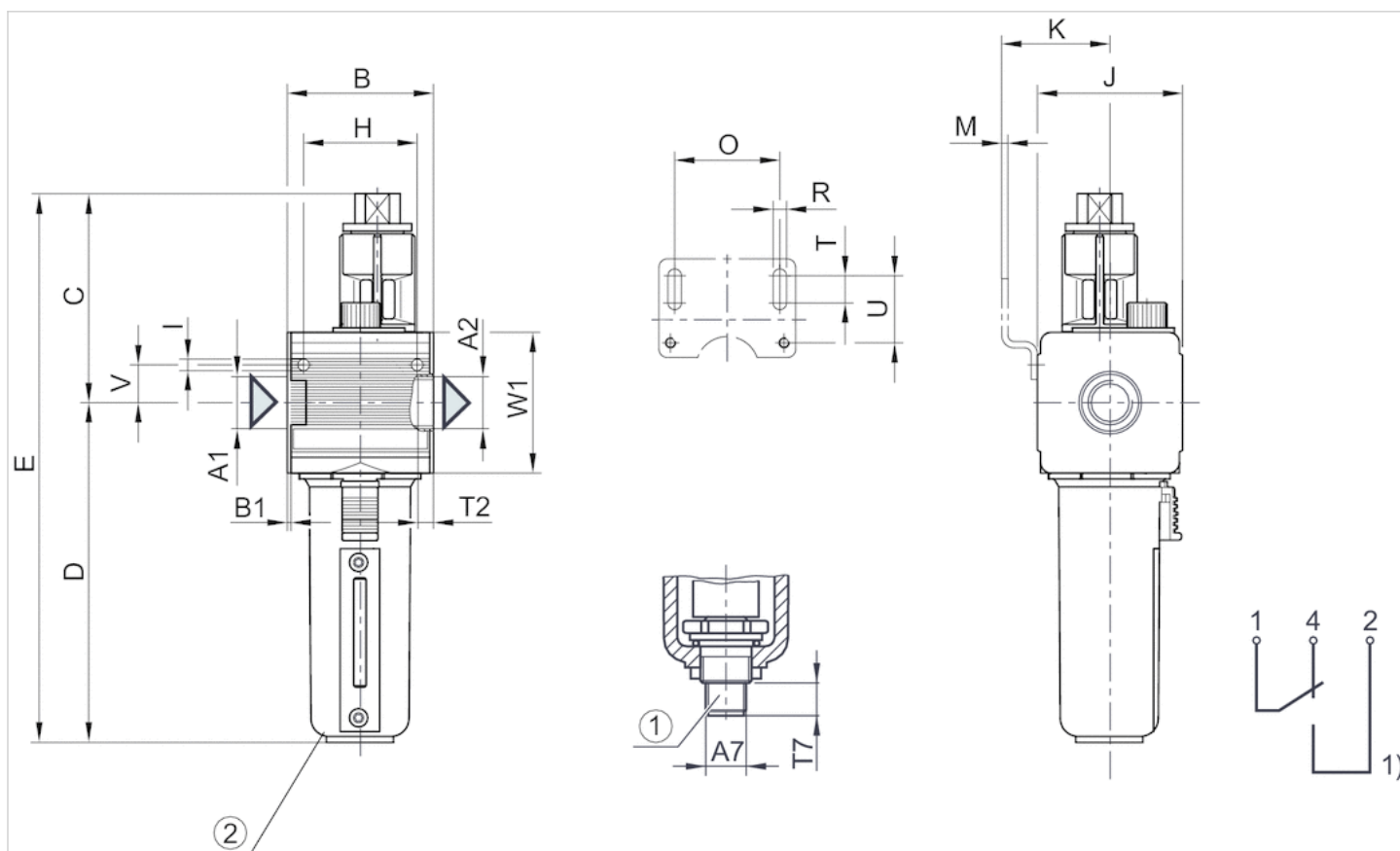
Fig. 2, Metal reservoir with level indicator
