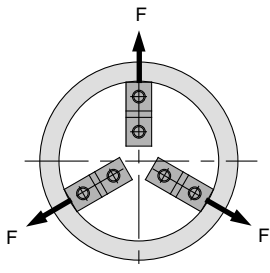
Internal gripping
