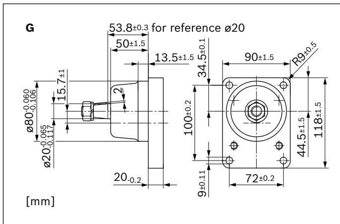
Outrigger bearing Ø80 mm, type 2
