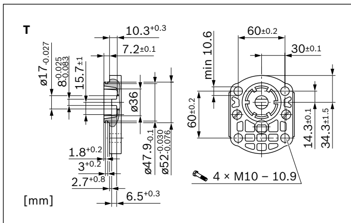
4-bolt mounting Ø52 mm, with O-ring
