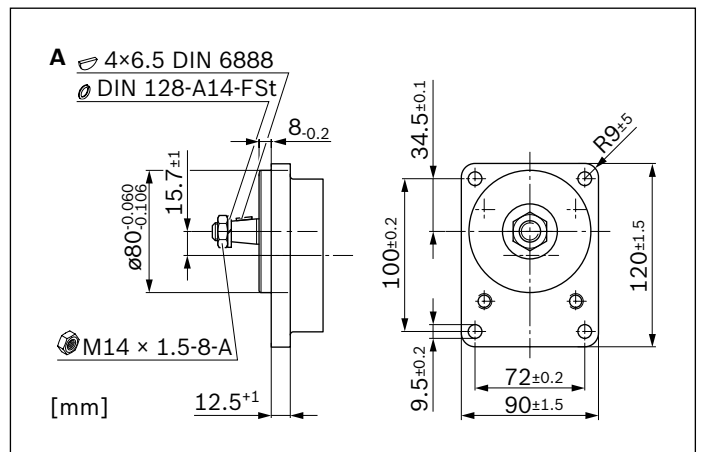
Outrigger bearing Ø80 mm, type 1
