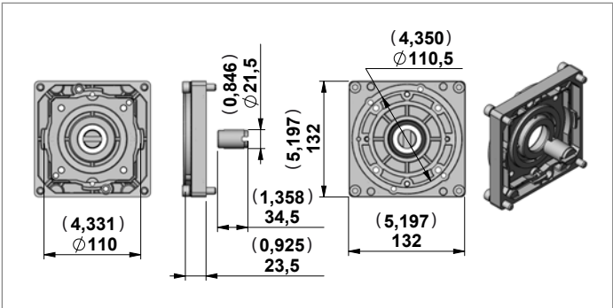
Junction Elements for manifolds KE and KS series
